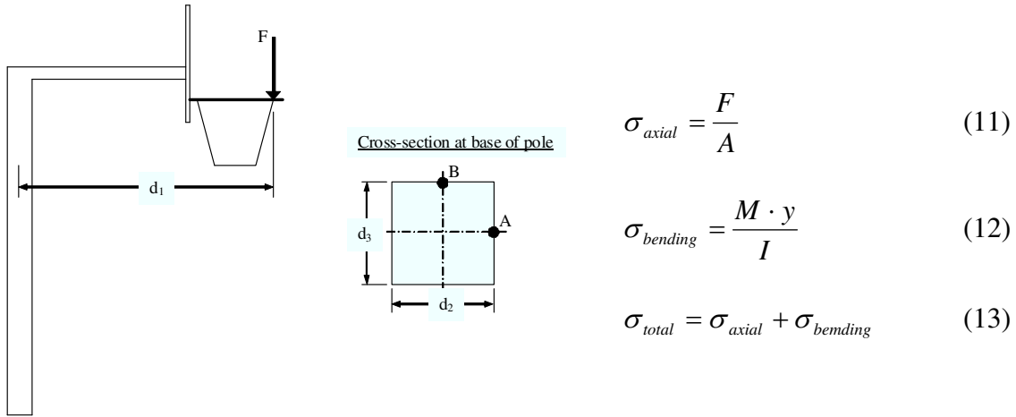
Figure 1: Stress Calculations for a Basketball Goal
